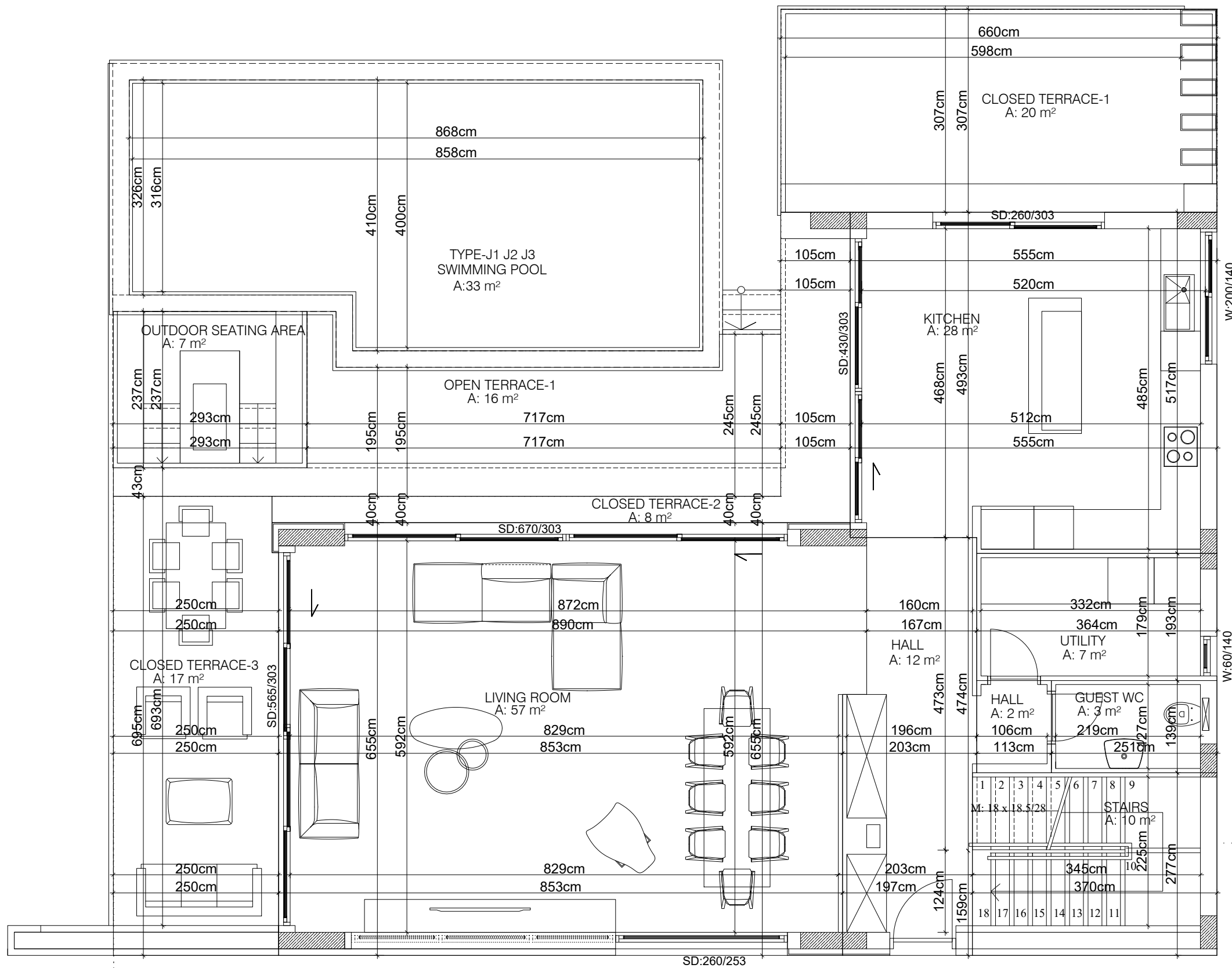
TYPE L1-L2 - GROUND FLOOR PLAN
