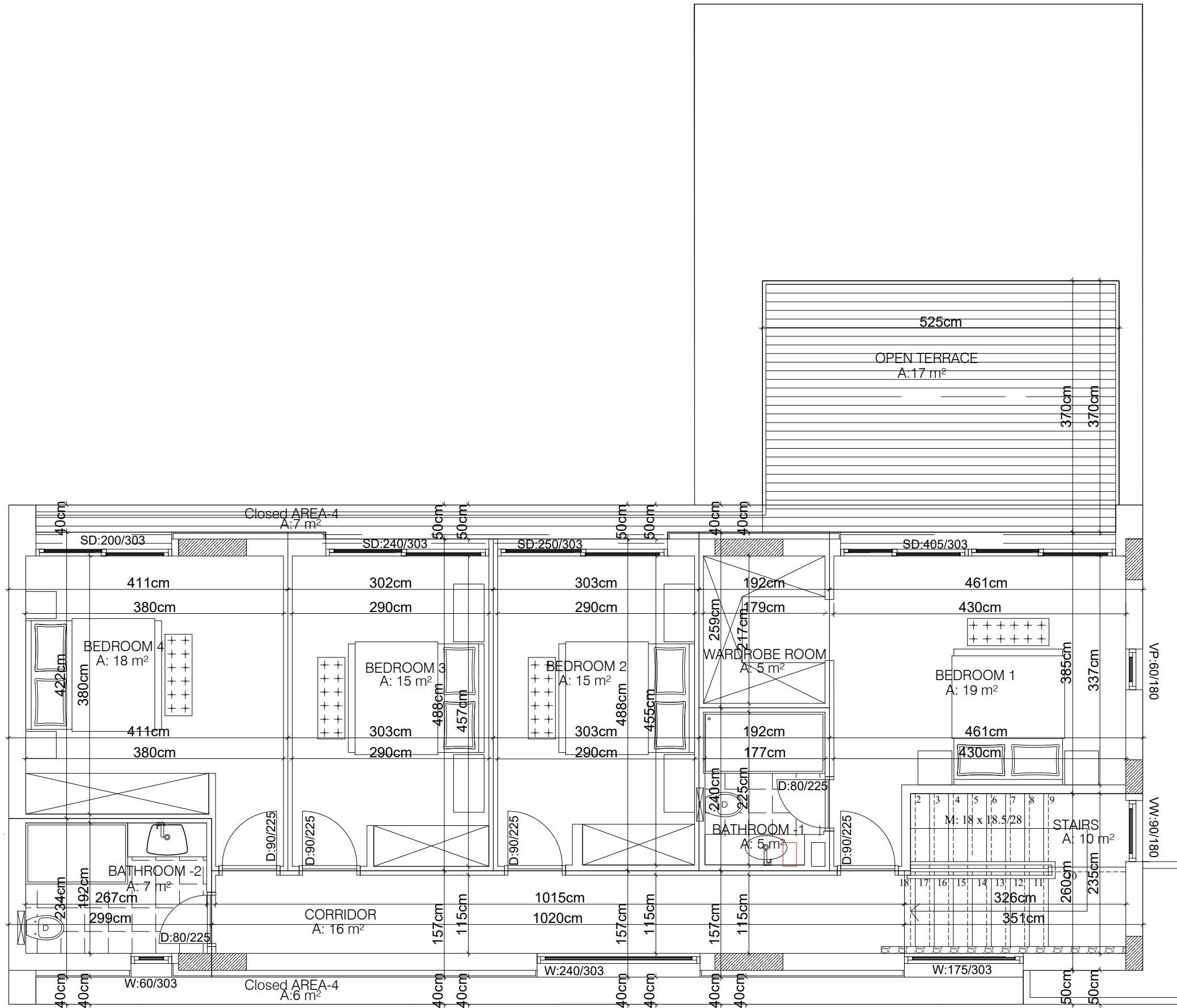
TYPE L1-L2 - 1. FLOOR PLAN
