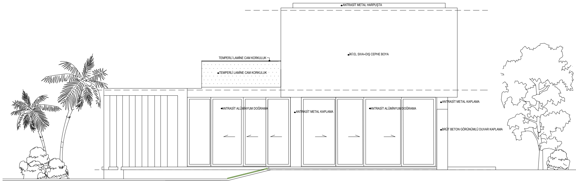
LEFT ELEVATION TYPE L1-L2
