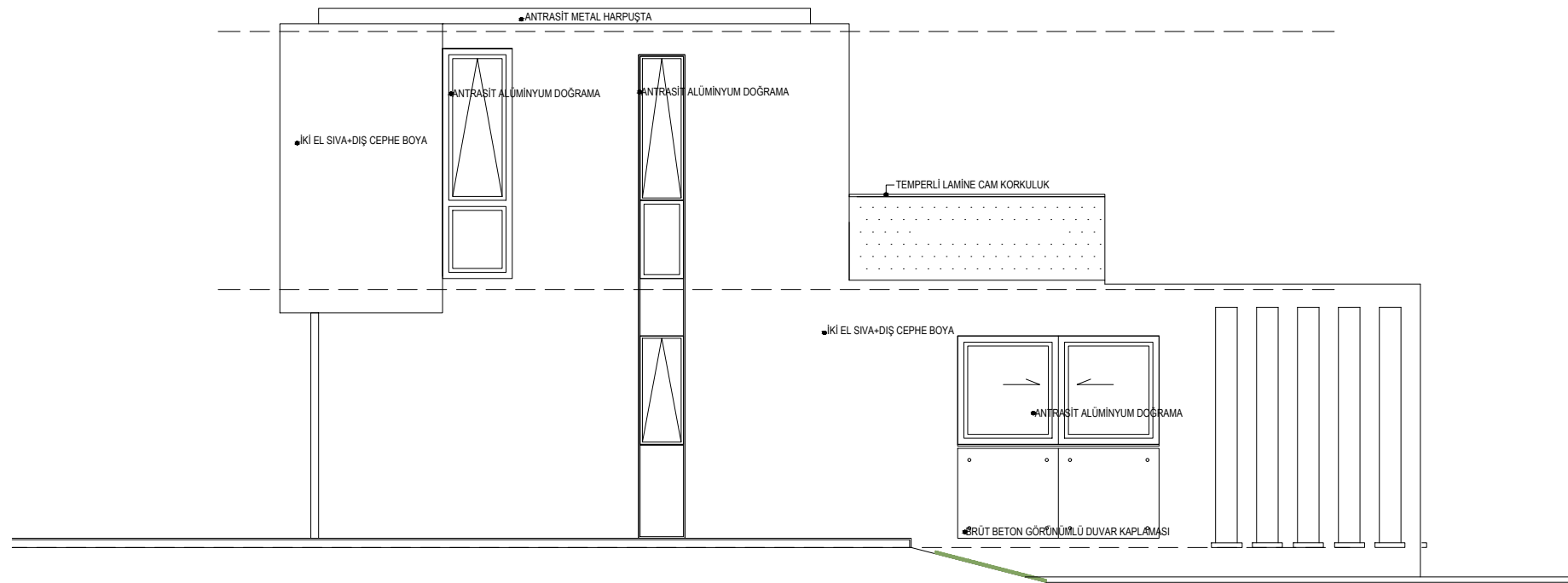
RIGHT ELEVATION TYPE L1-L2
