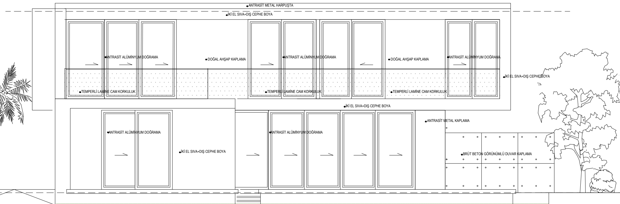
BACK ELEVATION TYPE L1-L2
